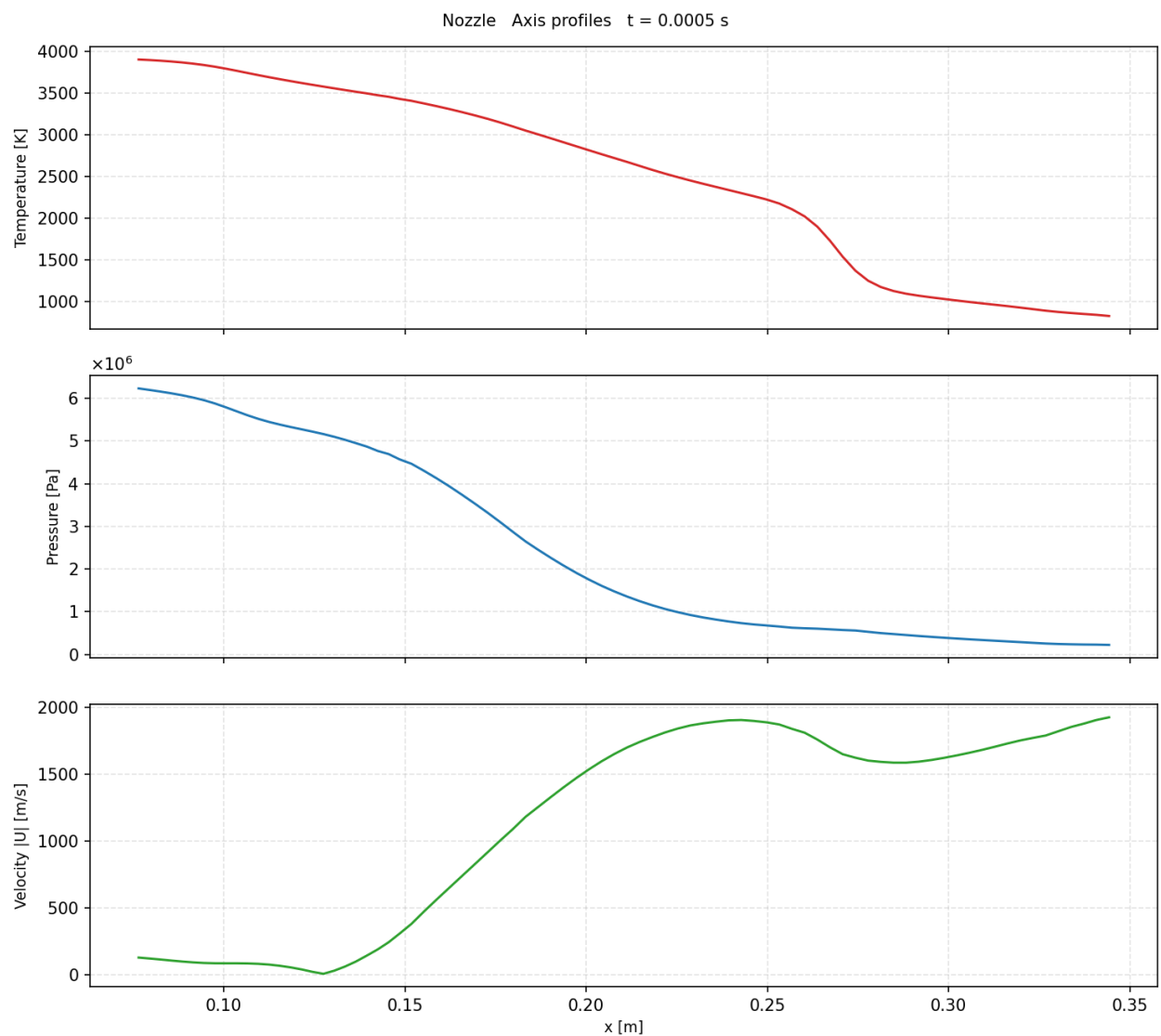
Fig. 5 — Axis profiles of T, p, |U| at t = 0.5 ms.
