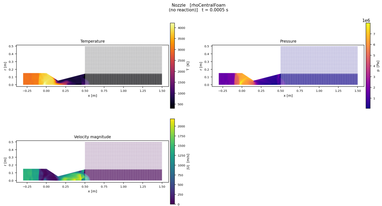
Fig. 4 — T, p, |U| at t = 0.5 ms (extended plume domain, startup transient).
