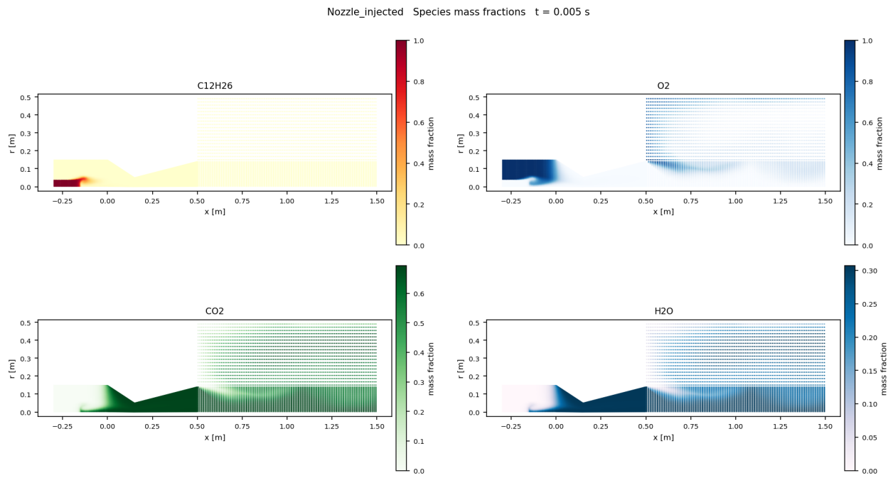
Fig. 10 — Mass fraction fields (C 12 H 26 , O 2 , CO 2 , H 2 O) at t = 0.005 s.
