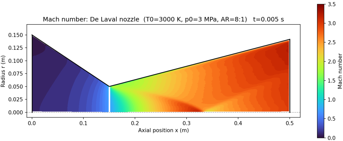
Fig. 3 — Mach number contour (nozzle-only domain, validated design point). Exit Mach \approx 3.22 matches isentropic theory (3.20) to within 1%.
